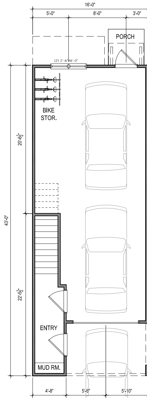
FIRST FLOOR PLAN 97 SF EXTERNAL HEATED 509 SF GARAGE
