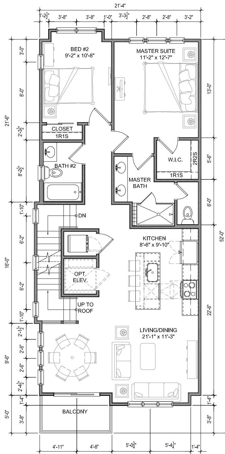
SECOND FLOOR PLAN 1,037 SF EXTERNAL HEATED 40 SF BALCONY
