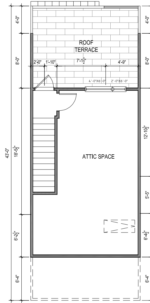
ATTIC PLAN 61 SF EXTERNAL HEATED 192 SF BALCONY
