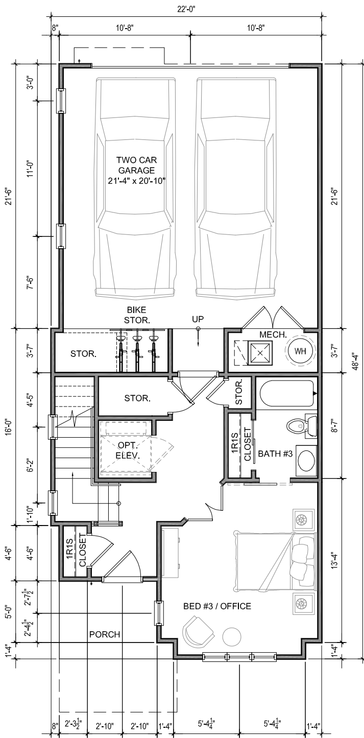
FIRST FLOOR PLAN 449 SF EXTERNAL HEATED 538 SF GARAGE
