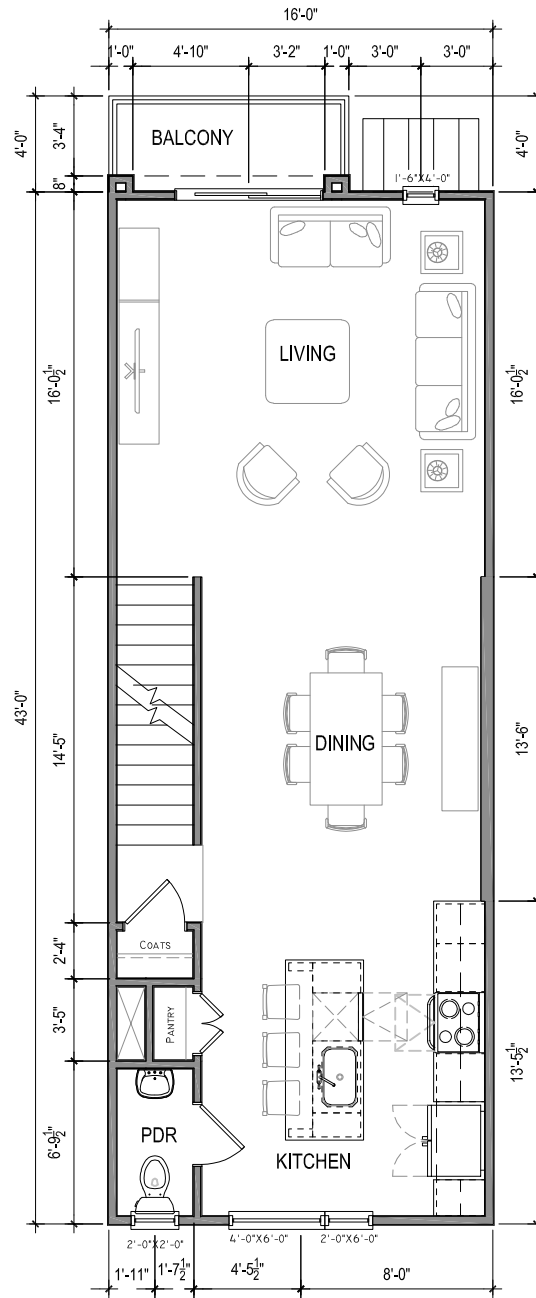
SECOND FLOOR PLAN 688 SF EXTERNAL HEATED 40 SF BALCONY
