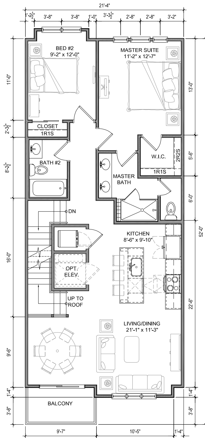
SECOND FLOOR PLAN 1,027 SF EXTERNAL HEATED 48 SF BALCONY
