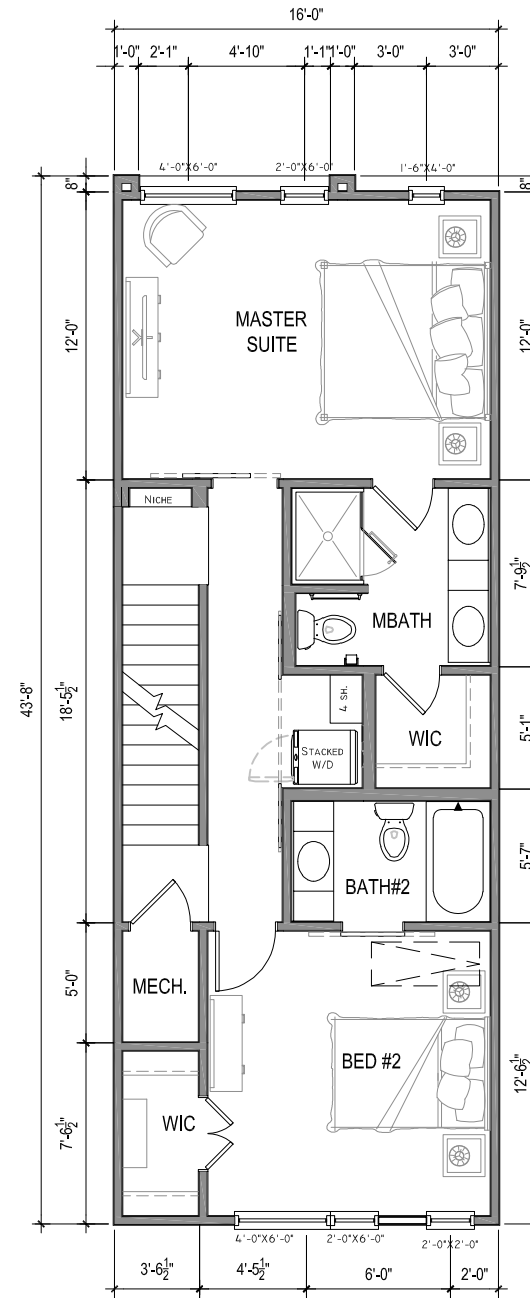
THIRD FLOOR PLAN 688 SF EXTERNAL HEATED
