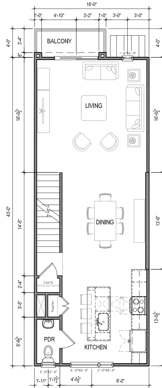
SECOND FLOOR PLAN 688 SF EXTERNAL HEATED 40 SF BALCONY
