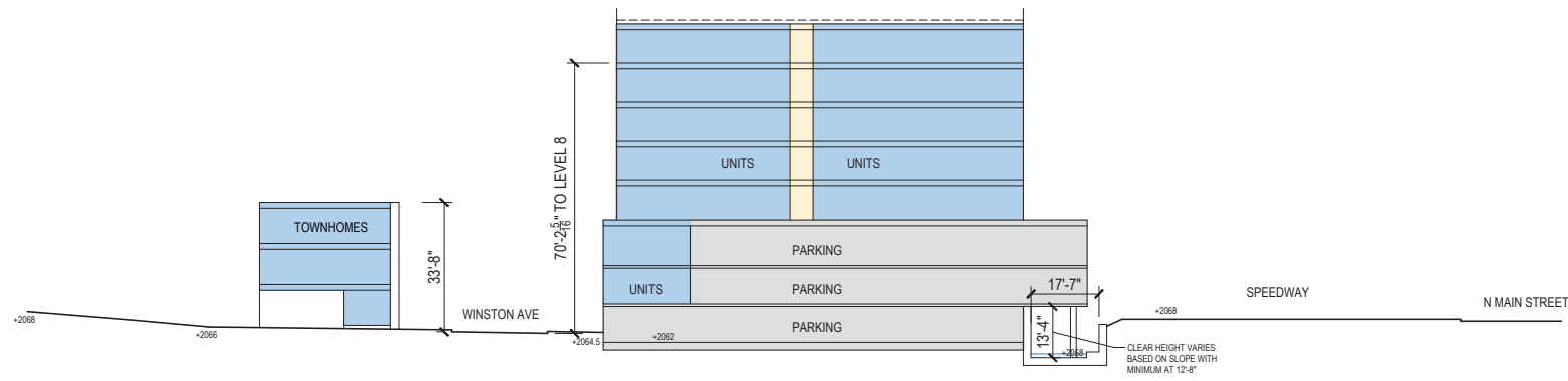
SECTION B
