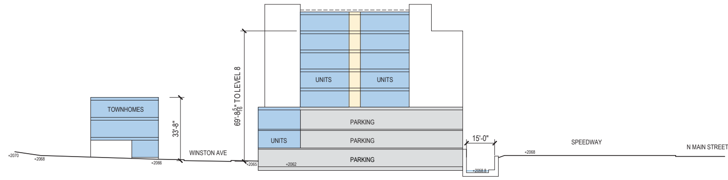
SECTION A
