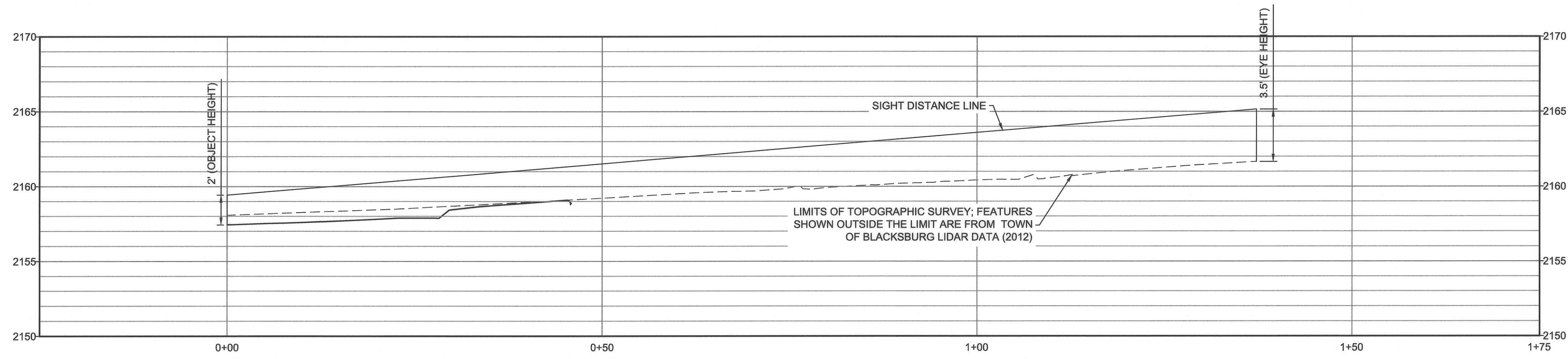
SIGHT DISTANCE PROFILE - Scale: H: 1"=10', V: 2.00:1
